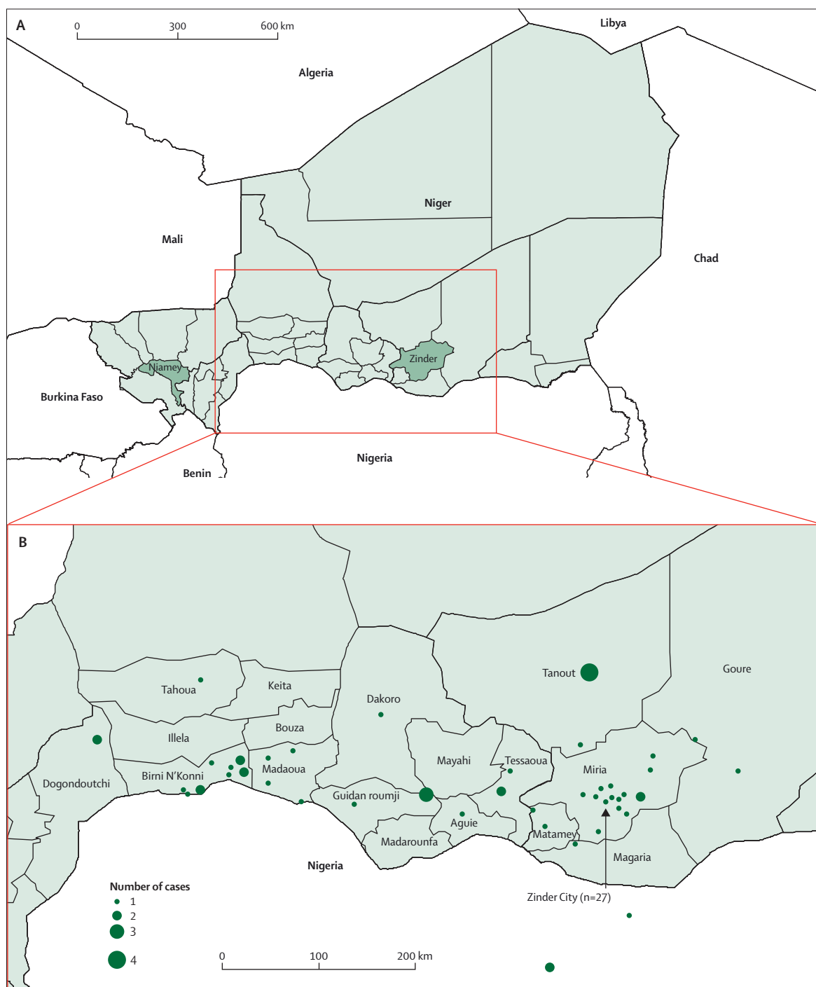
Figure 3: Geographical localisation of the study population, Zinder region, Niger, Africa (A) Niger (capital: Niamey) and surrounding African countries. (B) Geographical distribution of noma cases between Aug 1, 2001, and Oct 31, 2006, in the Zinder region of Niger
